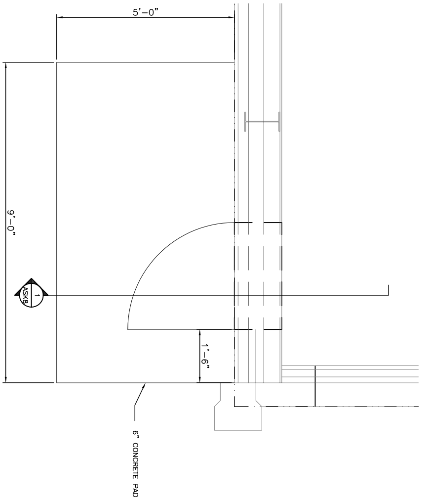
2 GYMNASIUM SOUTH WALL PLAN ASK#8 SCALE: 3/4" = 1'-0"
